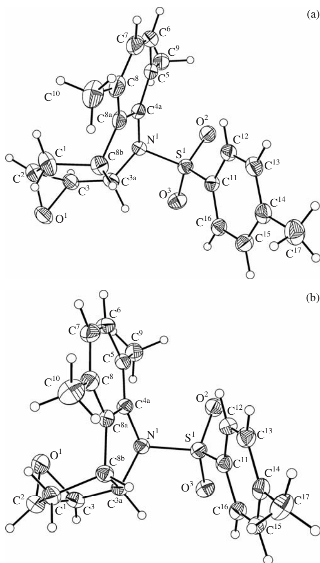
Fig. 1. Structures of molecules (a) XIII f and (b) XIV f according to the X-ray diffraction data. Non-hydrogen atoms are shown as thermal ellipsoids with a probability of 50%.
